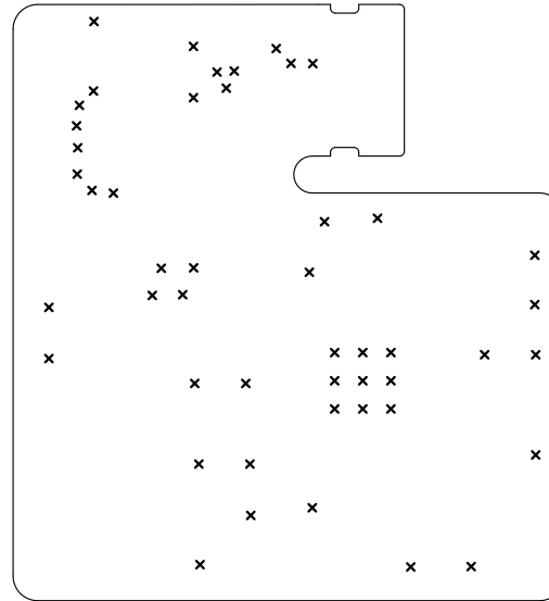
Drill Map: × 0.300mm / 0.0118" (48 holes)
